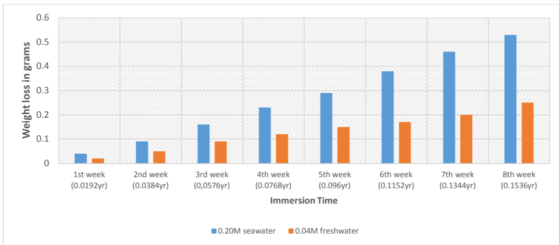
Fig. 4. Weight loss results of coupons in 0.2 M of seawater and 0.04M of freshwater exposed for eight weeks against time
