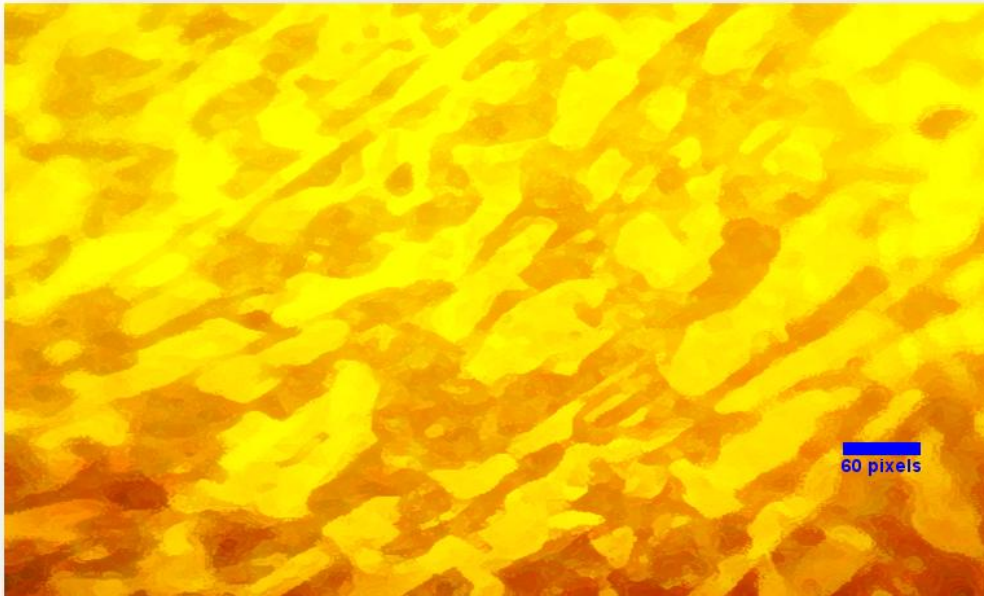
Fig. 6. Micrograph of coupon 2 before immersion X 400 in 0.2M of seawater
