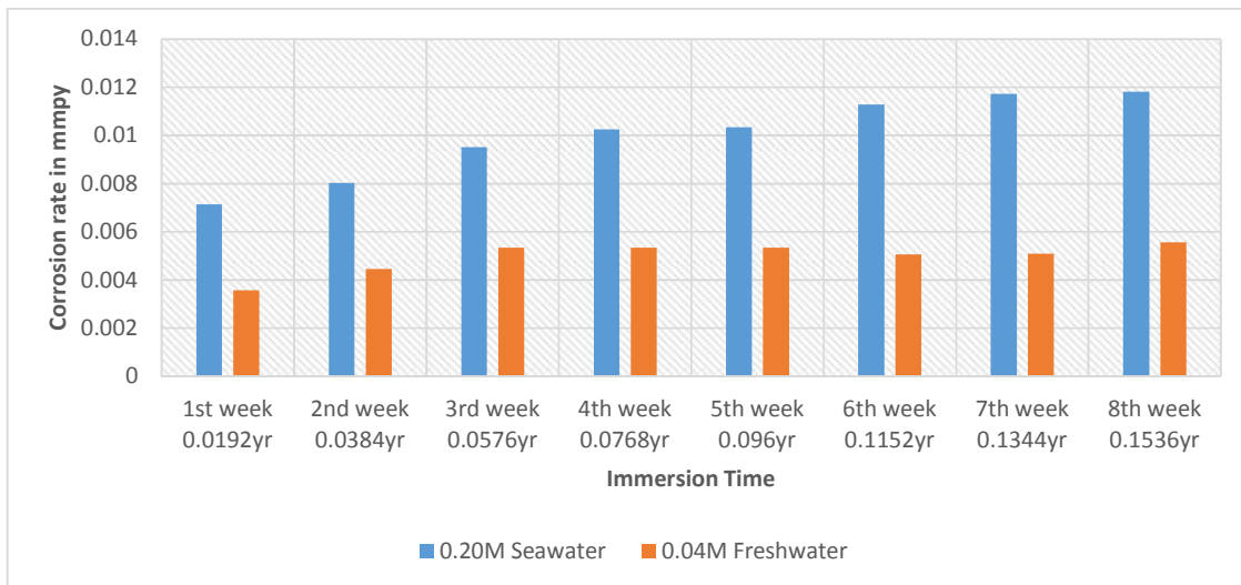
Fig. 5. Corrosion rate results of coupon 2 in 0.2 M of seawater and coupon 1 in 0.04 M of freshwater exposed for eight weeks against Time
