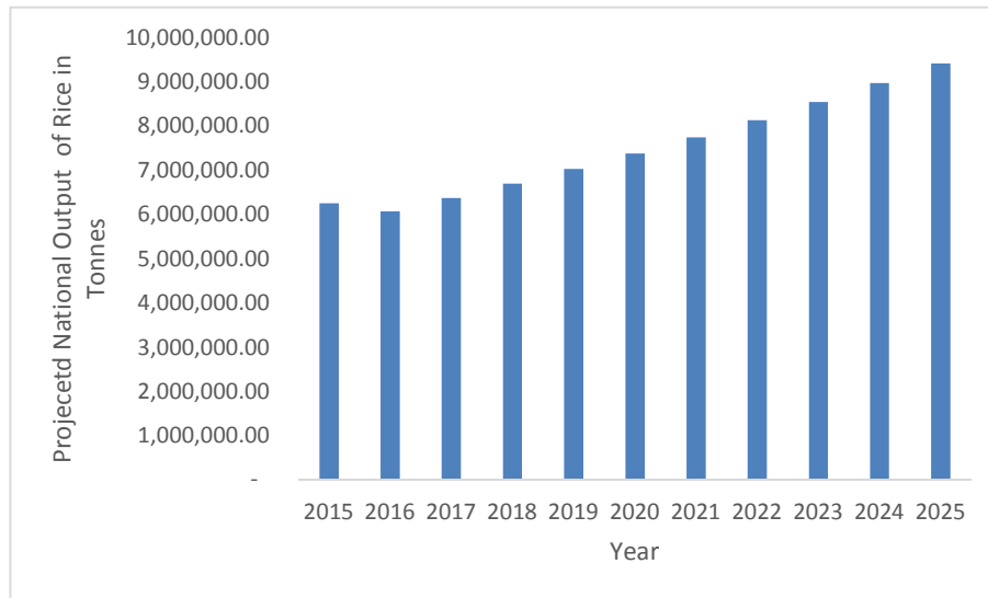
Fig. 3. Projected national output of paddy-rice from 2017-2025
