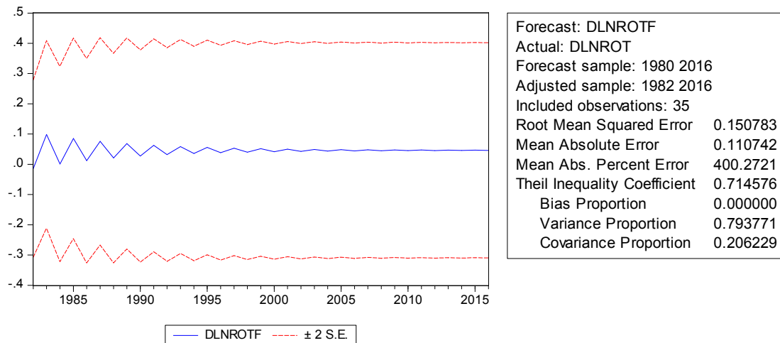
Fig. 2. Ex post prediction (model validation)
