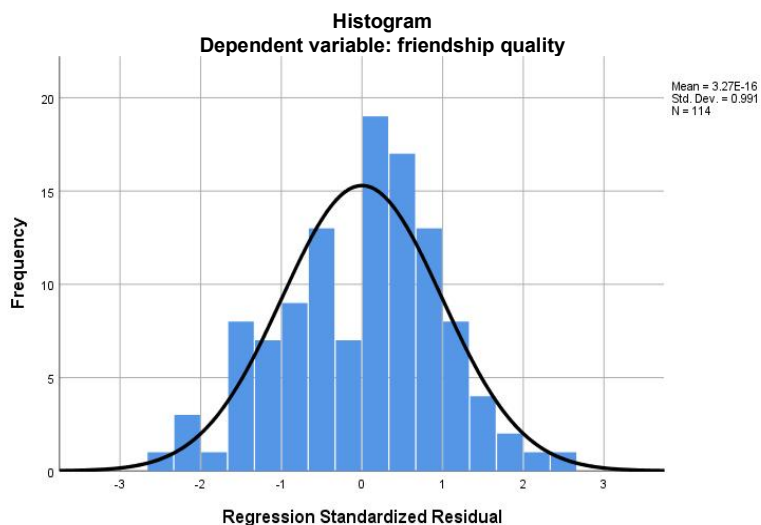
Fig. 2 Normal distribution curve
