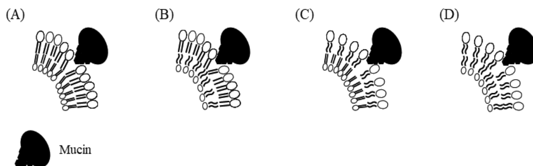
Fig. 3. Mucin effect on lipid layer. Outer layer is exposed to mucin. (A) Both solids, (B) Solid outer-layer, (C) Liquid outer-layer, and (D) Both liquids
