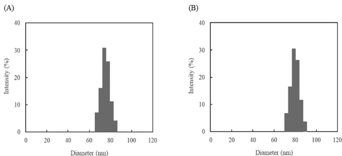
Fig. 1. Diameter data of (A) micelles and (B) vesicles
