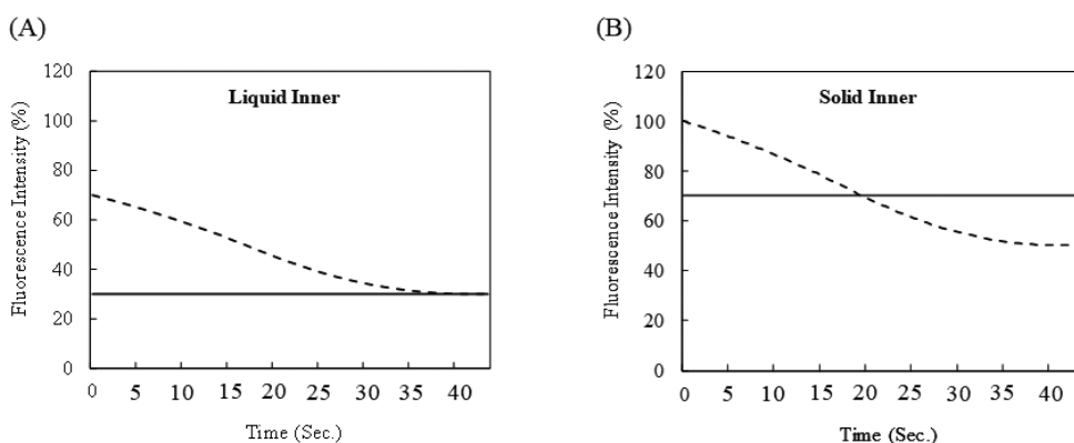
Fig. 2. Fluorescence intensity of vesicles with solid outer (---) and with liquid outer (—) at 0.5 ratio. (A) liquid inner and (B) solid inner
