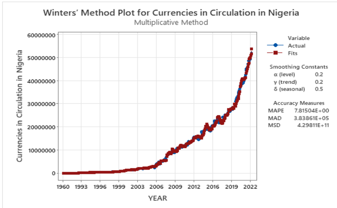
Fig. 3. Multiplicative Holt–Winters method with \alpha= 0.2 , \gamma= 0.2 , \delta= 0.5
