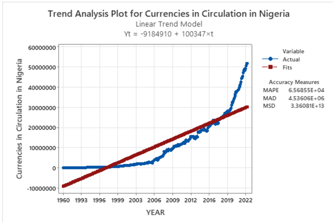
Fig. 1. Trend analysis plot for currencies in circulation in Nigeria
