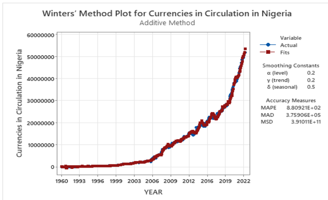
Fig. 4. Additive Holt–Winters model with \alpha= 0.2 , \gamma= 0.2 , \delta= 0.5
