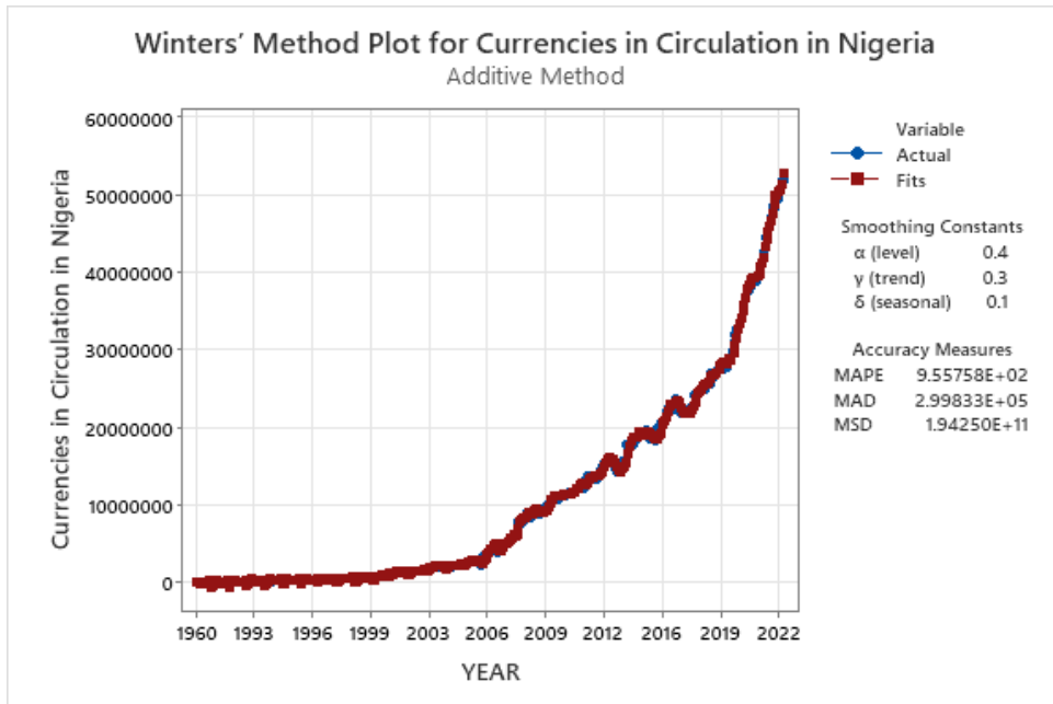
Fig. 10. Additive Holt–Winters model with \alpha= 0.4 , \gamma= 0.3 , \delta= 0.1
