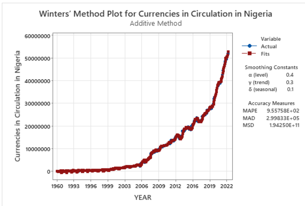
Fig. 6. Additive Holt–Winters model with \alpha= 0.4, \gamma= 0.3, \delta= 0.1
