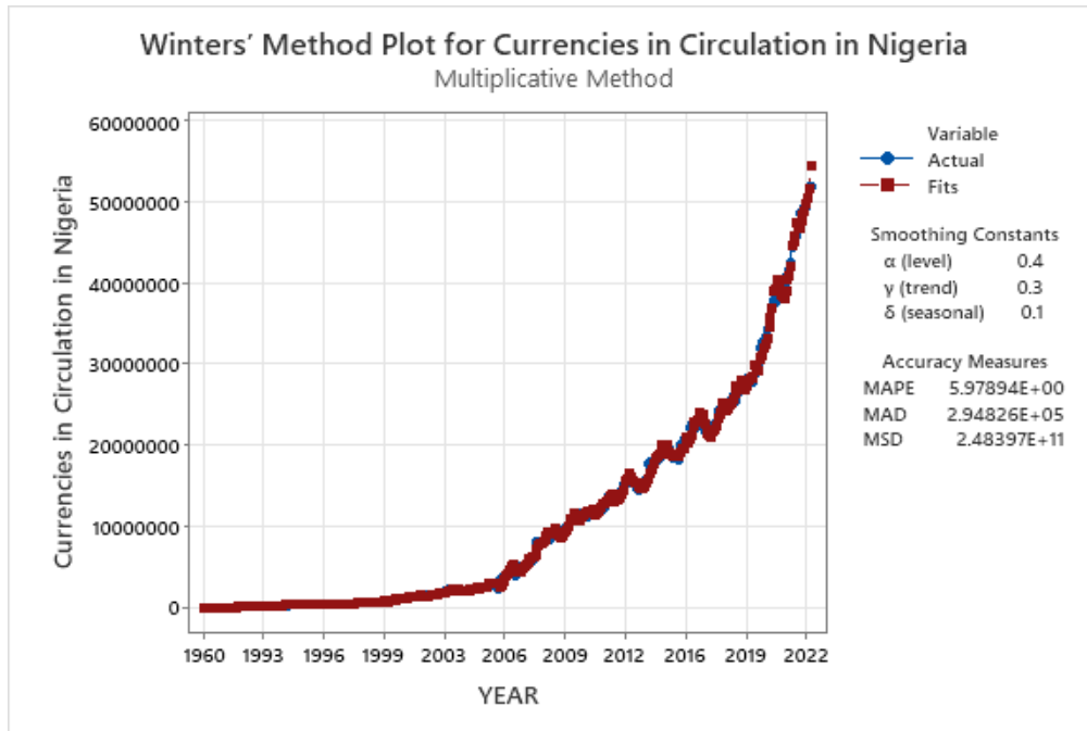
Fig. 5. Multiplicative Holt–Winters method with \alpha= 0.4, \gamma= 0.3, \delta= 0.1
