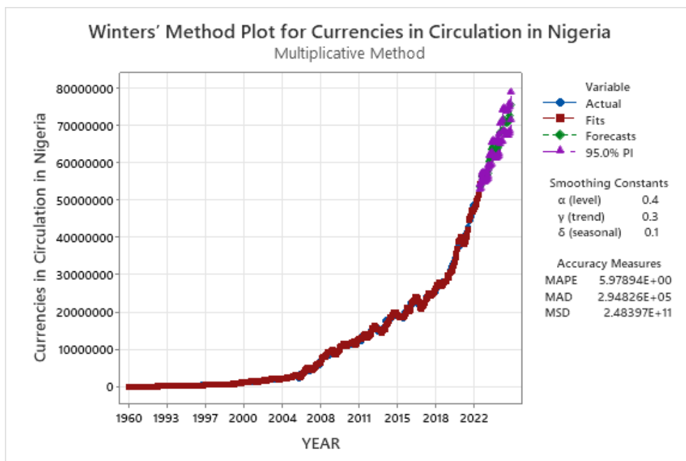
Fig. 11. Forecast of currencies in circulation in Nigeria using multiplicative method
