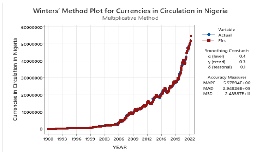
Fig. 9. Multiplicative Holt–Winters method with \alpha= 0.4, \gamma= 0.3, \delta= 0.1
