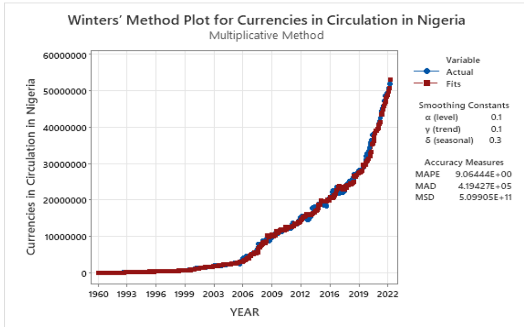
Fig. 7. Multiplicative Holt–Winters method with \alpha=0.1 , \gamma=0.1 , \delta=0.3
