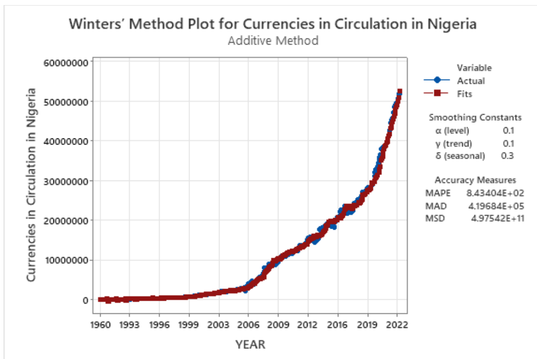
Fig. 8. Additive Holt–Winters model with \alpha=0.1 , \gamma=0.1 , \delta=0.3
